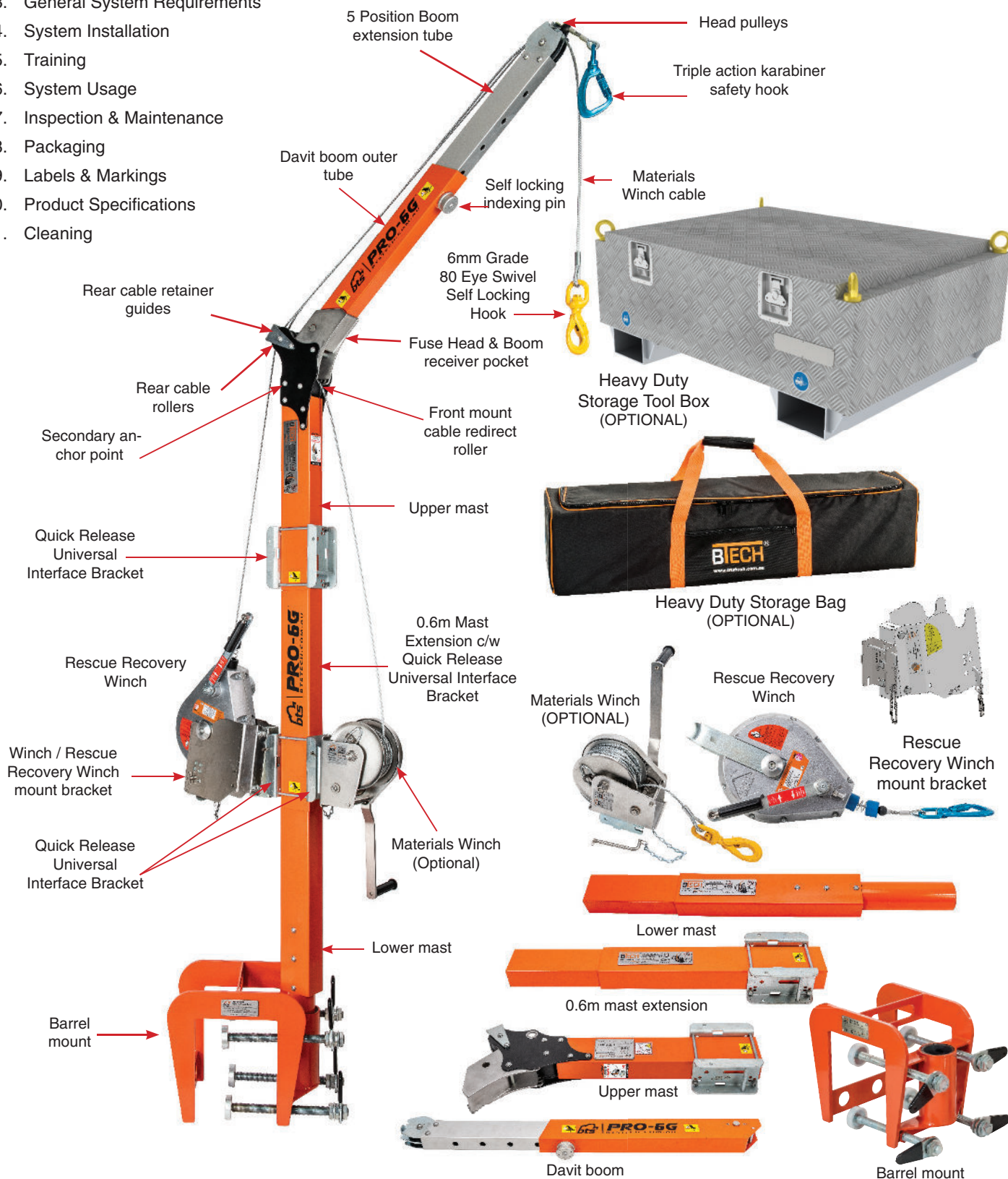
Figure 1. Parts
